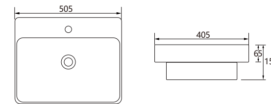
DUI4940 SEMI-INSET GLOSS WHITE 1 TAP HOLE 32MM WASTE WITH OVERFLOW
