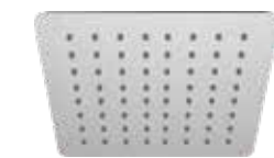
Item Code T-SB2125 - BN Description 250mm x 250mm Square Raincloud Shower Head - Brushed Nickel WATER RATING 3 STAR, 9.0L/MIN
