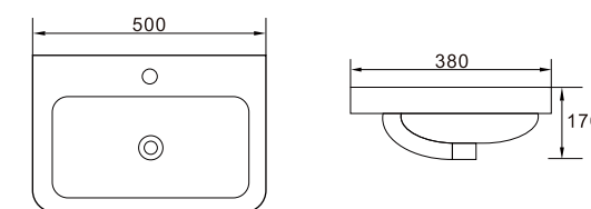
DJ5038 INSET BASIN GLOSS WHITE 1 TAP HOLE 32MM WASTE WITH OVERFLOW
