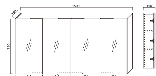
Item Code M-DUS15-O Description 1500 shaving cabinet 1500 x 150 x 720 - Oak
