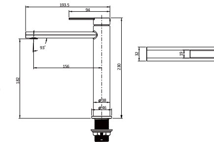
Item Code T-SBMH T-SBMH-B T-SBMH-BN T-SBMH-BG Description Serena Tall Basin Mixer Serena Tall Basin Mixer - Matte Black Serena Tall Basin Mixer - Brush Nickel Serena Tall Basin Mixer - Brush Gold Water Rating 4 Star, 6.5 L/MIN
