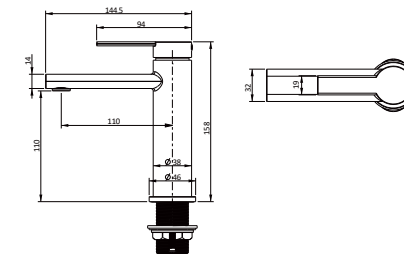
Item Code T-SBM T-SBM-B T-SBM-BN T-SBM-BG Description Serena Basin Mixer Serena Basin Mixer - Matte Black Serena Basin Mixer - Brush Nickel Serena Basin Mixer - Brush Gold Water Rating 4 Star, 6.5 L/MIN
