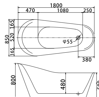
MODEL: VU182-1800 size: 1800x850x800mm
