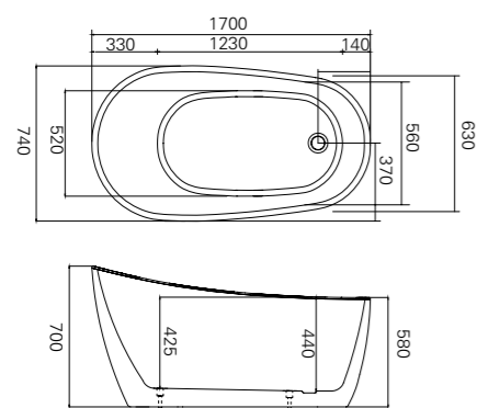
MODEL: VU899-170 size: 1700x740x700mm
