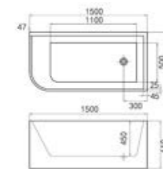
MODEL: VU754R-1500 size: 1500x750x610mm
