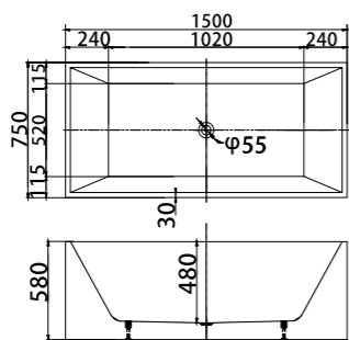
MODEL: VU708 -1500 size: 1500x750x580mm
