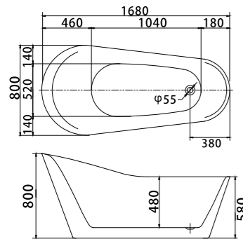
MODEL: VU182-1700 size: 1680x800x800mm
