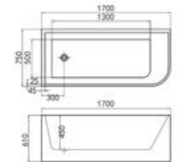
MODEL: VU754L-1700 size: 1700x750x610mm
