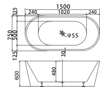
MODEL: VU816-1500 size: 1500x750x600mm
