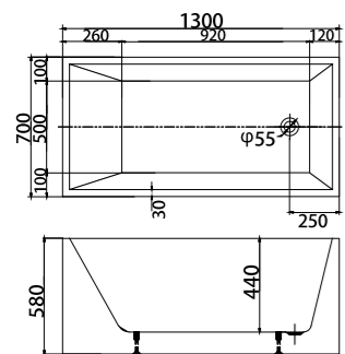
MODEL: VU708 -1300 size: 1300x700x580mm
