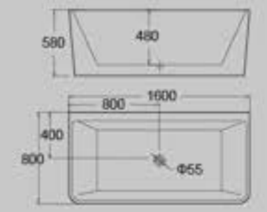
MODEL: VU720 size: 1600x800x580mm
