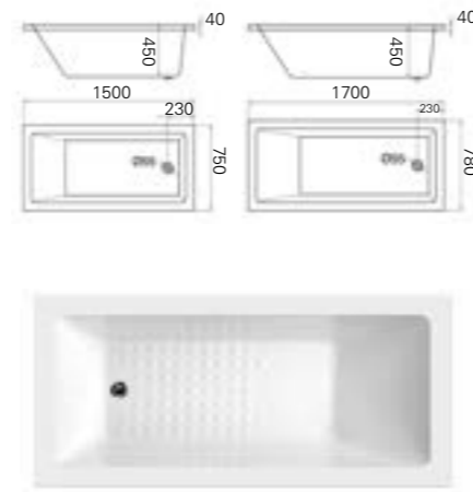
MODEL: VY-1700 size:1700x780x450mm
