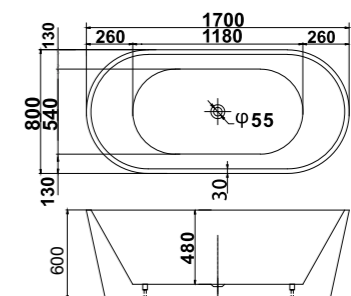
MODEL: VU816-1700 size: 1700x800x600mm
