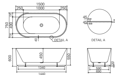
MODEL: VU537-1500 size: 1500x750x600mm
