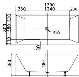
MODEL: VU708 -1700 size: 1700x800x580mm
