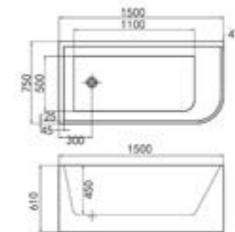
MODEL: VU754L-1500 size: 1500x750x610mm
