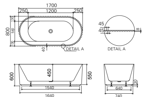
MODEL: VU537-1700 size: 1700x800x600mm
