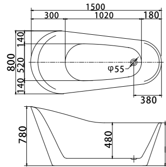
MODEL: VU182-1500 size: 1500x800x780mm
