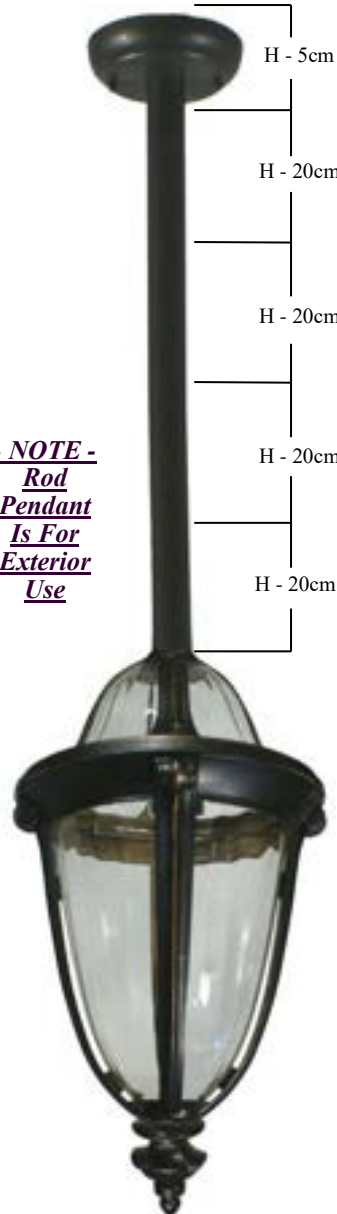
1000313 MAYFAIR ROD PND E27 FRAME SIZE H - 49cm W - 26cm + 4 x 20cm RODS + 1 x 5cm CAP
