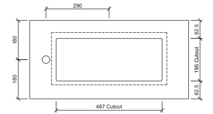
Taphole Offset
