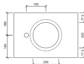
Taphole Offset
