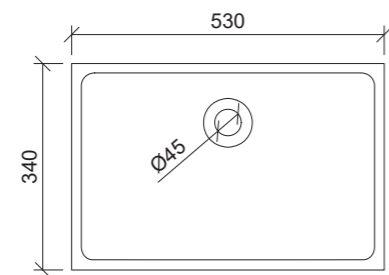
Taphole Offset
