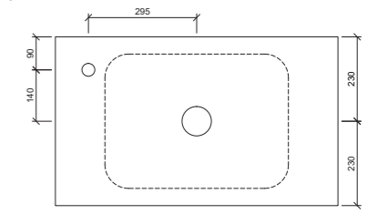
Taphole Offset
