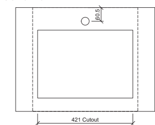
Taphole Behind
