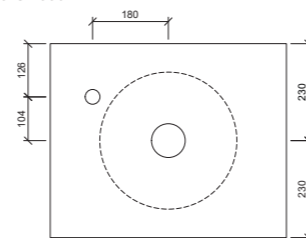
Taphole Behind
