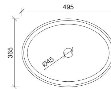
Taphole Offset
