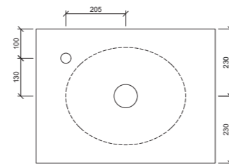
Taphole Offset
