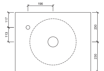
Taphole Offset
