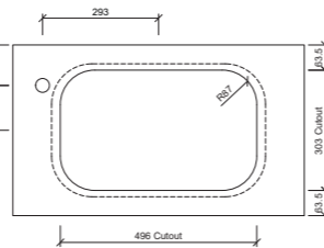
Taphole Offset
