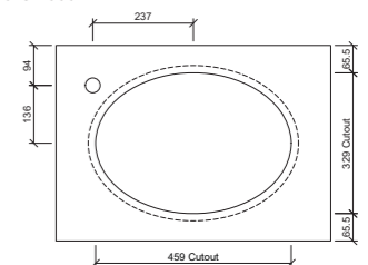
Taphole Offset
