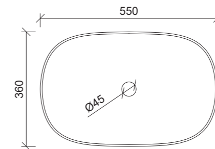
Taphole Offset
