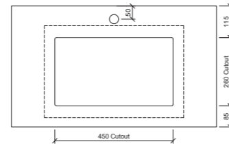
Taphole Behind
