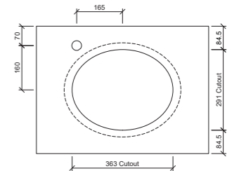
Taphole Behind
