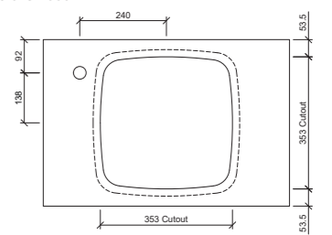
Taphole Offset
