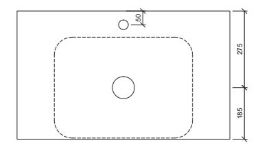
Taphole Behind
