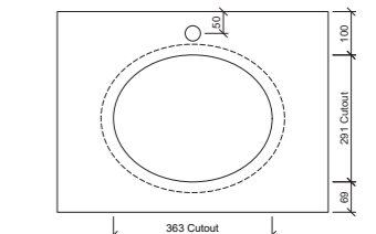
Taphole Behind
