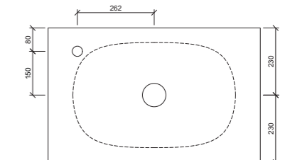
Taphole Offset
