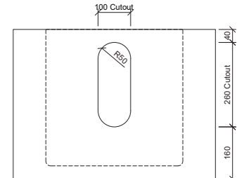
Taphole Offset
