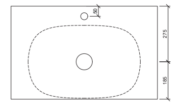
Taphole Behind
