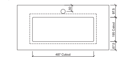
Taphole Behind
