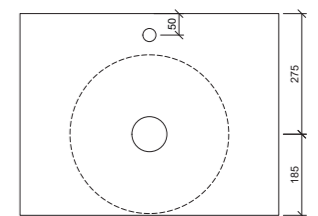
Taphole Behind
