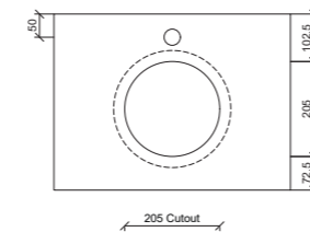
Taphole Behind
