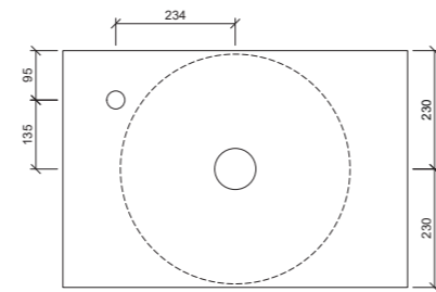
Taphole Offset
