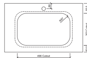
Taphole Behind
